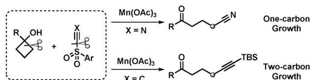
Scheme 1. Manganese-catalyzed ring-opening functionalization of cyclobutanol substrates. TBS = tert -butyldimethylsilyl.
