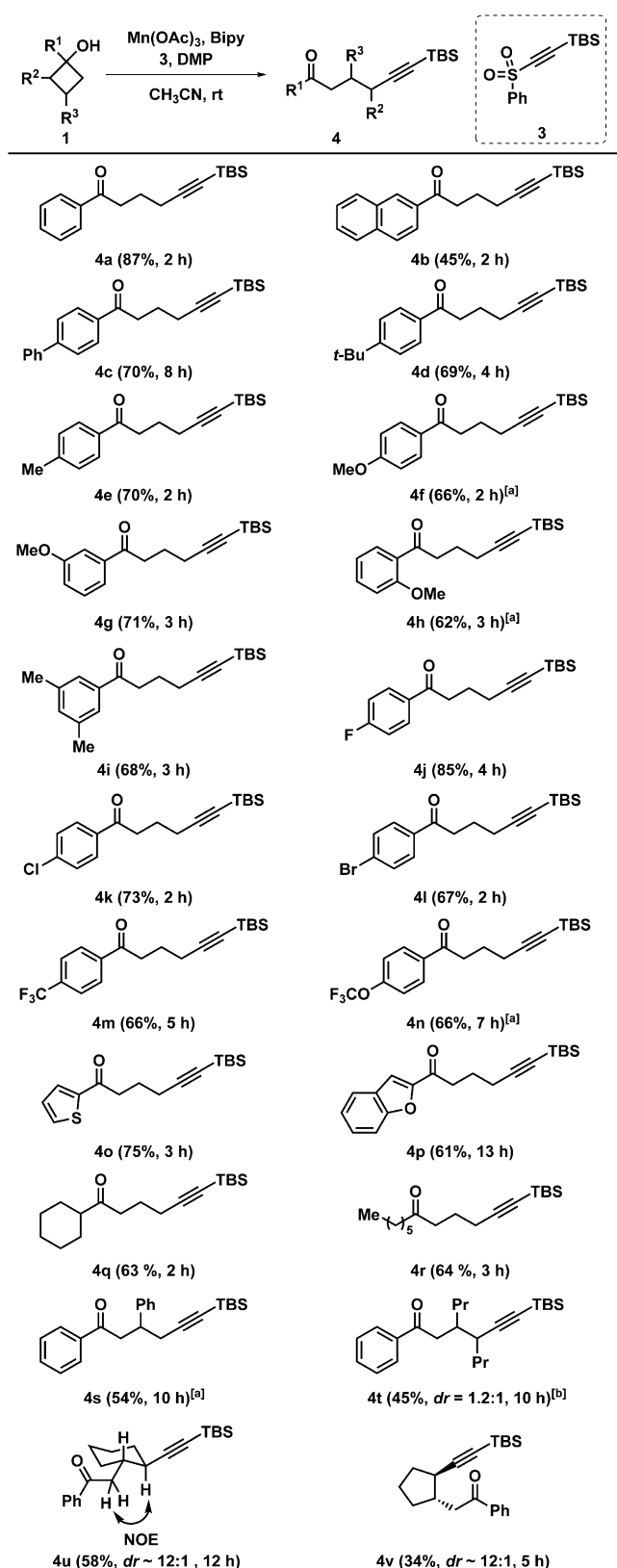
Scheme 3. Ring-opening ethynylation of tert -cyclobutanol substrates. Reaction conditions: 1 (0.20 mmol), 3 (0.30 mmol, 1.5 equiv), Mn(OAc) 3 ·2H 2 O (0.04 mmol, 0.2 equiv), bipy (0.044 mmol, 0.22 equiv), and DMP (0.40 mmol, 2.0 equiv) in CH 3 CN (1.5 mL) at RT. Yields of isolated products are given. [a] PIDA (2.0 equiv) was used instead of DMP. [b] Mn(OAc) 3 ·H 2 O (1.5 equiv) was used instead of the combination of Mn(OAc) 3 ·H 2 O, bipy, and DMP.
