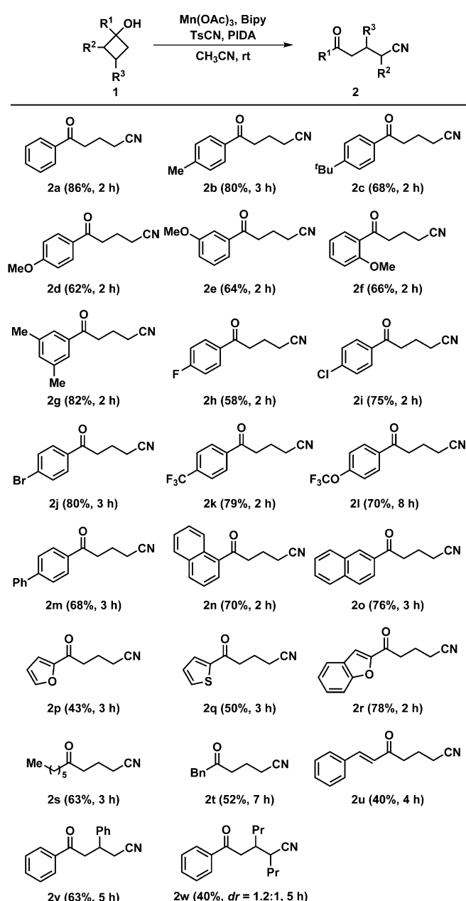
Scheme 2. Ring-opening cyanation of tert -cyclobutanol substrates. Reaction conditions: 1 (0.20 mmol), TsCN (0.30 mmol, 1.5 equiv), Mn(OAc) 3 ·2 H 2 O (0.04 mmol, 0.2 equiv), bipy (0.044 mmol, 0.22 equiv), and PIDA (0.40 mmol, 2.0 equiv) in CH 3 CN (1.5 mL) at RT. Yields of isolated products are given.
