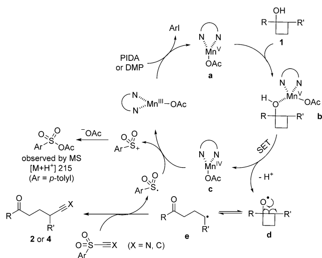
Figure 1. Plausible mechanistic pathway.
