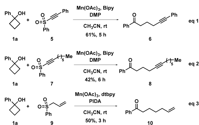
Scheme 4. Other examples of ring-opening C–C bond formation.
